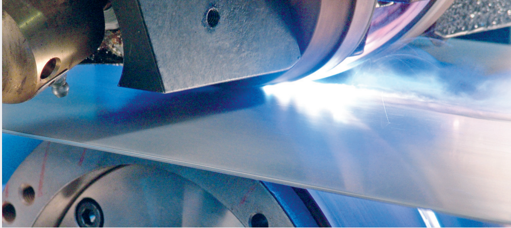
Welding the starting material
